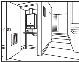
Closet Installation of GWH 425 PN with proper venting and combustion air supply shown.
